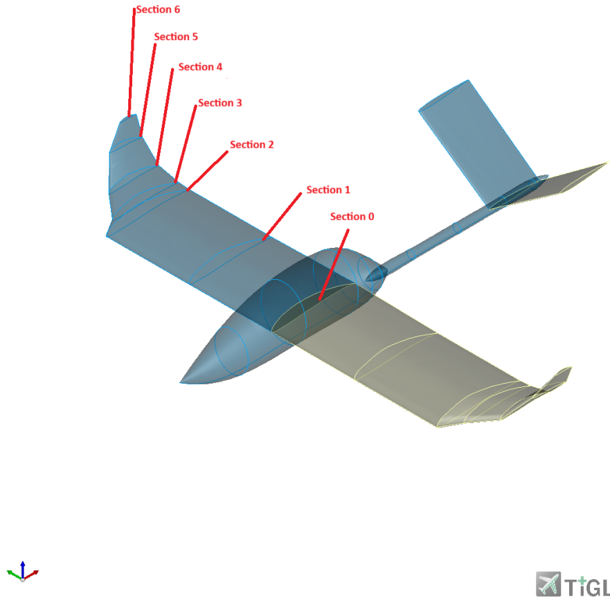
Figure 3.2: Wing Sections.
