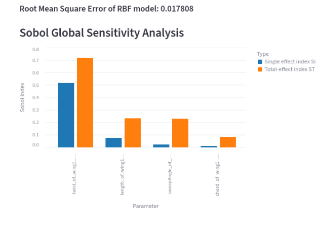
Figure 4.6: Results page: Sobol analysis.
